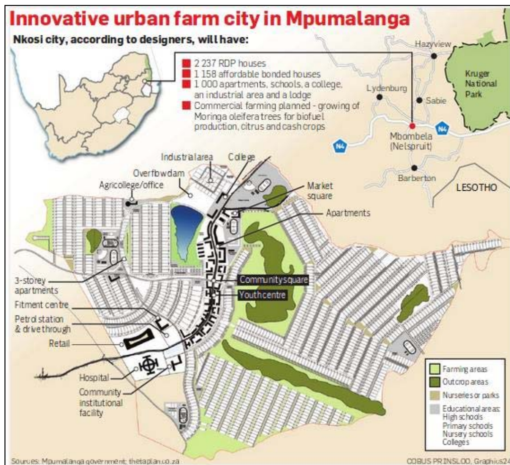
Figure 3-1: Proposed Nkosi City Layout
