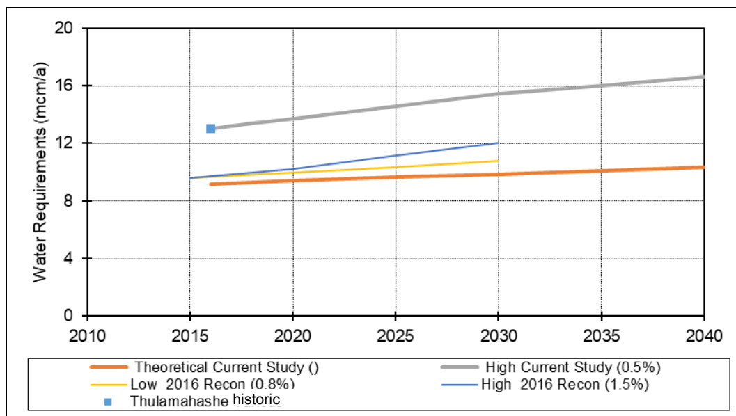
Figure 3-10: Water Requirements Projection for Thulamahashe Demand Centre
