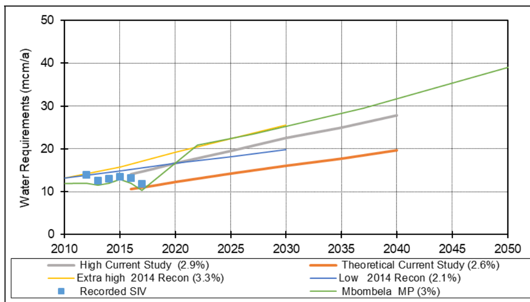
Figure 3-3: Water Requirements Projection for Mbombela
