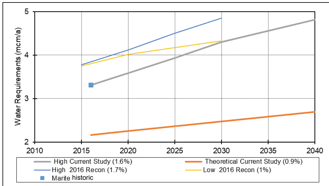
Figure 3-9: Water Requirements Projection for the Marite Demand Centre
