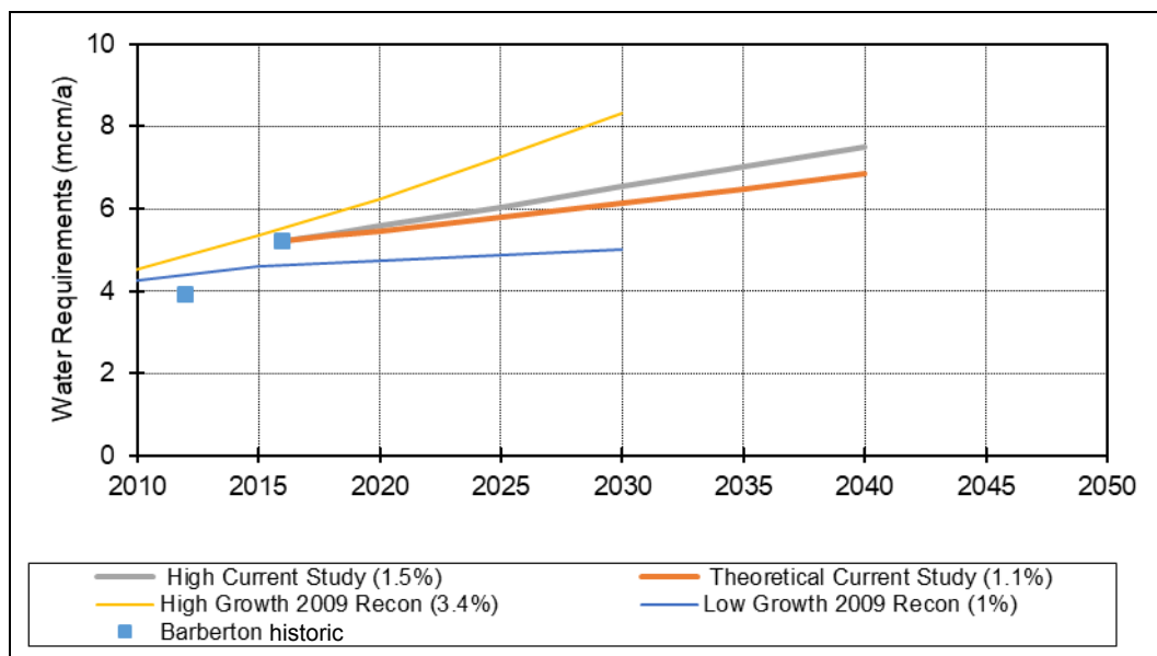
Figure 3-7: Water Requirements Projection for Barberton
