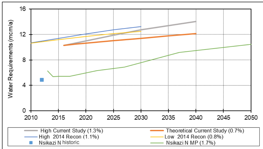
Figure 3-4: Water Requirements Projection for Nsikazi North
