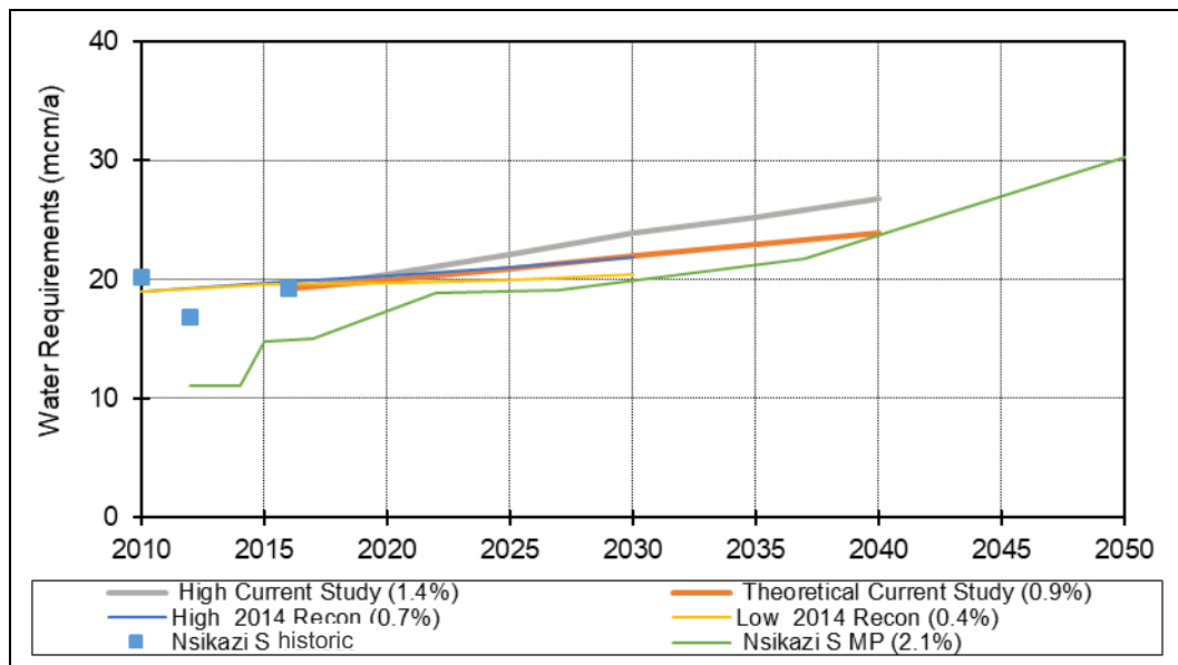
Figure 3-5: Water Requirements Projection for Nsikazi South
